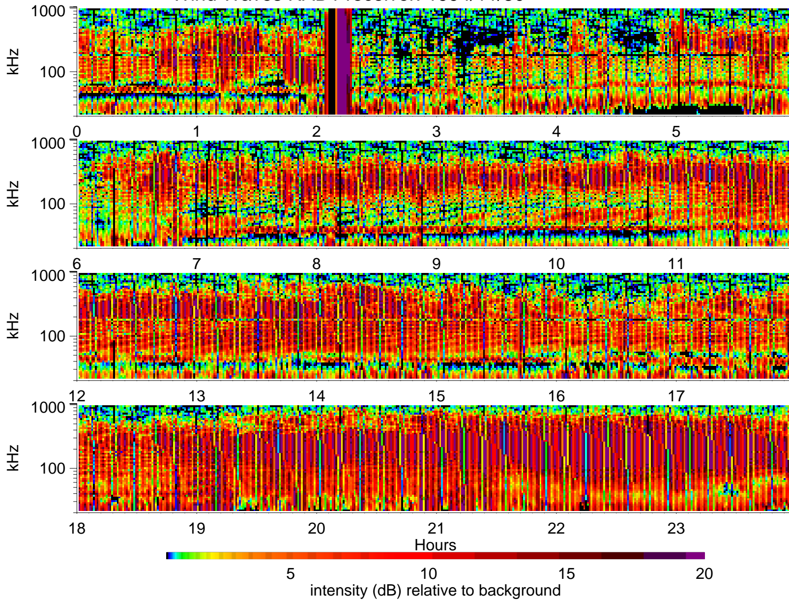
Wind Waves RAD1 receiver: 1994/11/30
