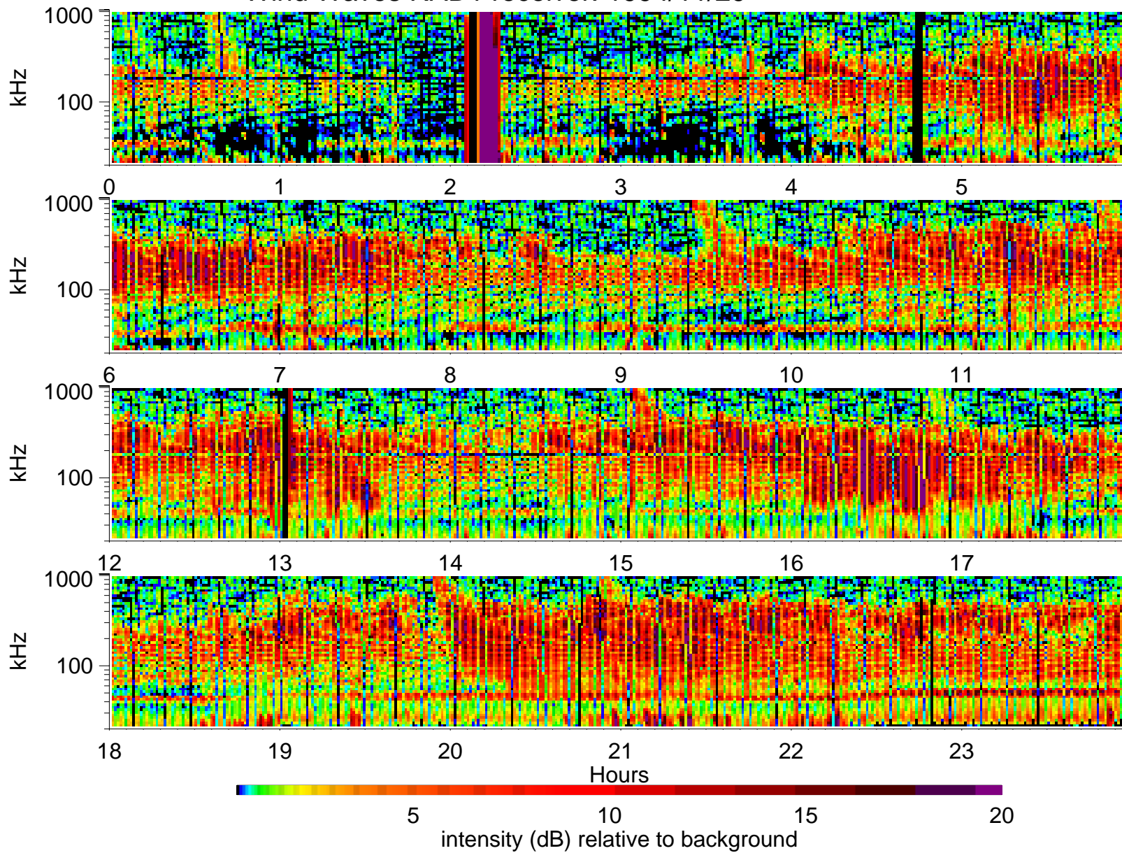
Wind Waves RAD1 receiver: 1994/11/29
