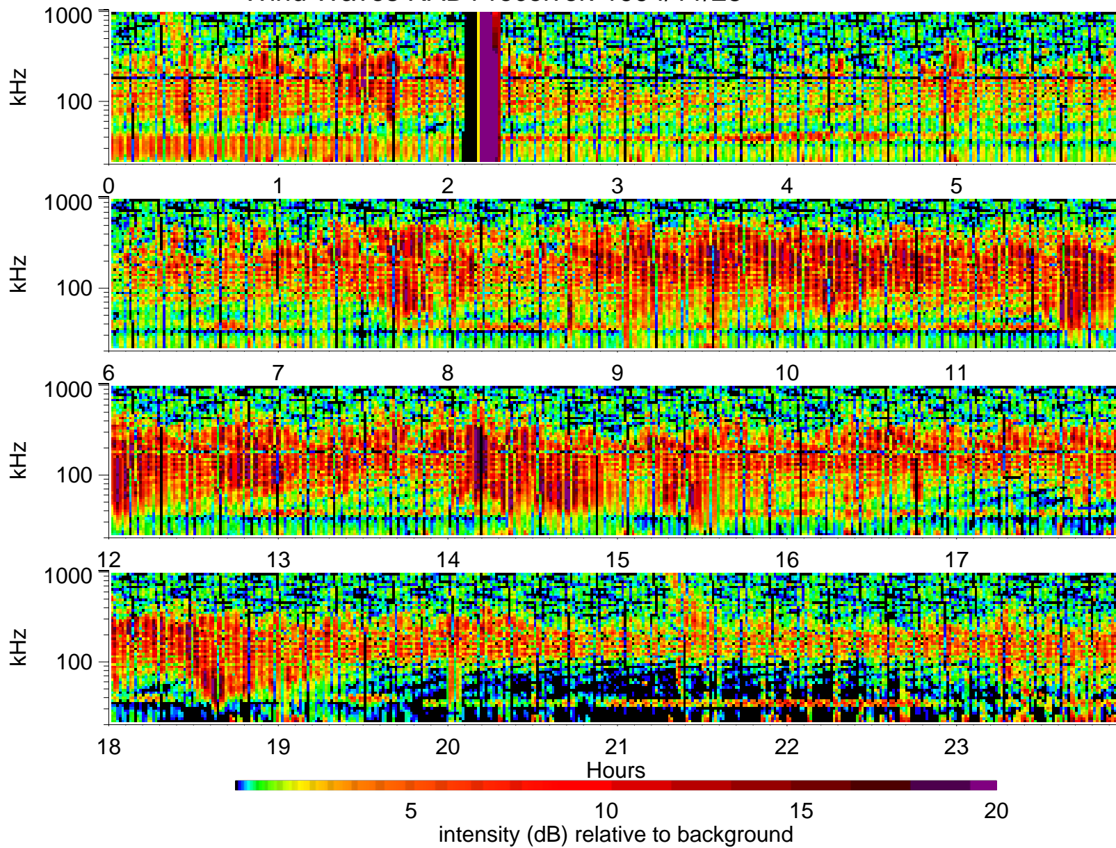
Wind Waves RAD1 receiver: 1994/11/28
