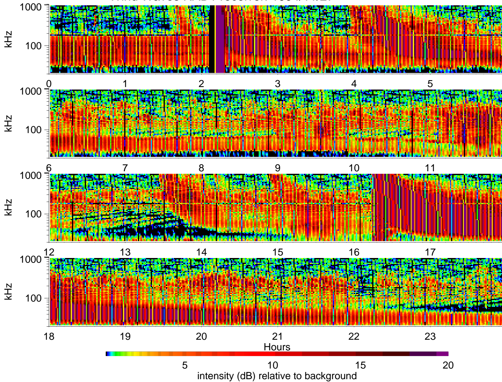
Wind Waves RAD1 receiver: 1994/11/27
