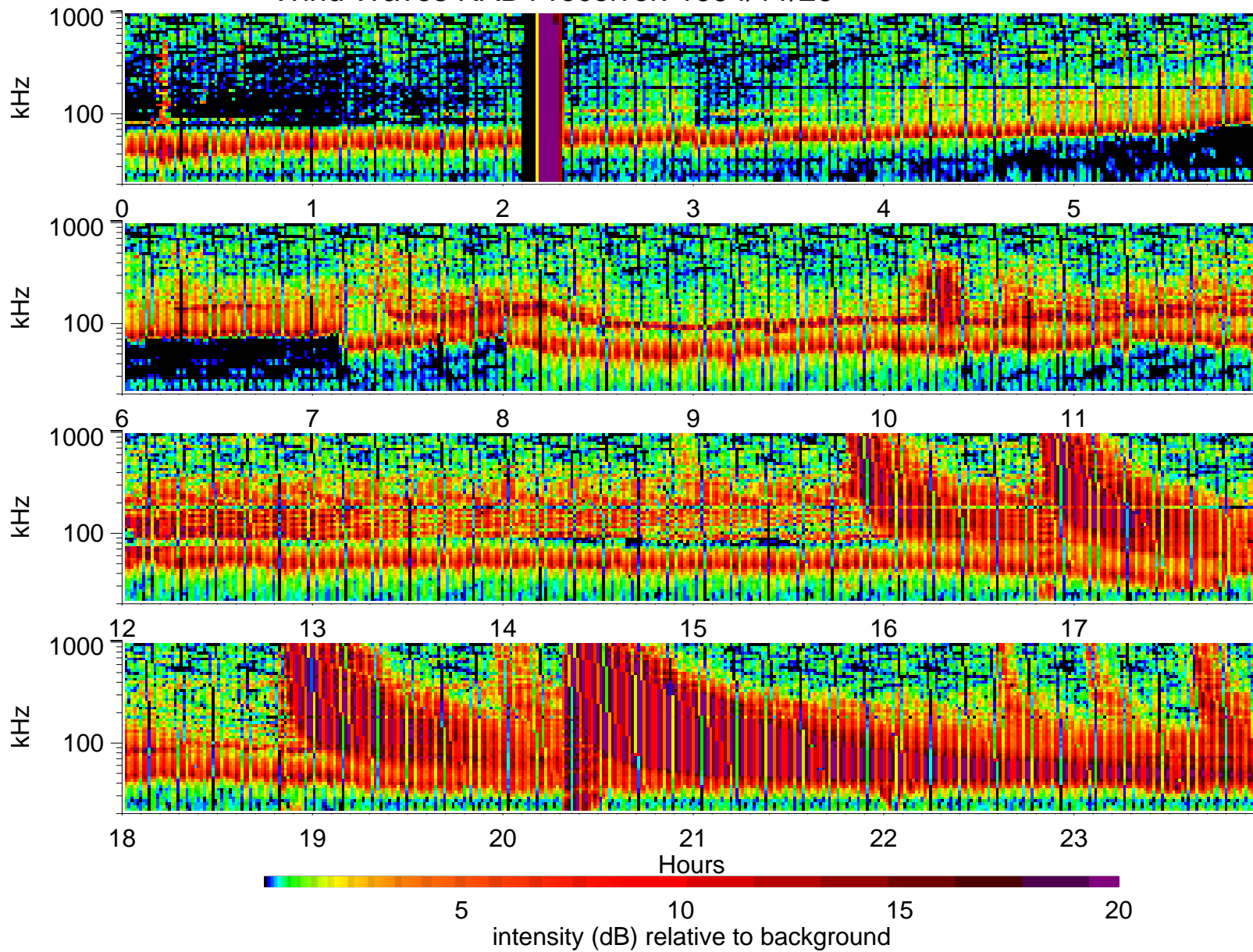
Wind Waves RAD1 receiver: 1994/11/26
