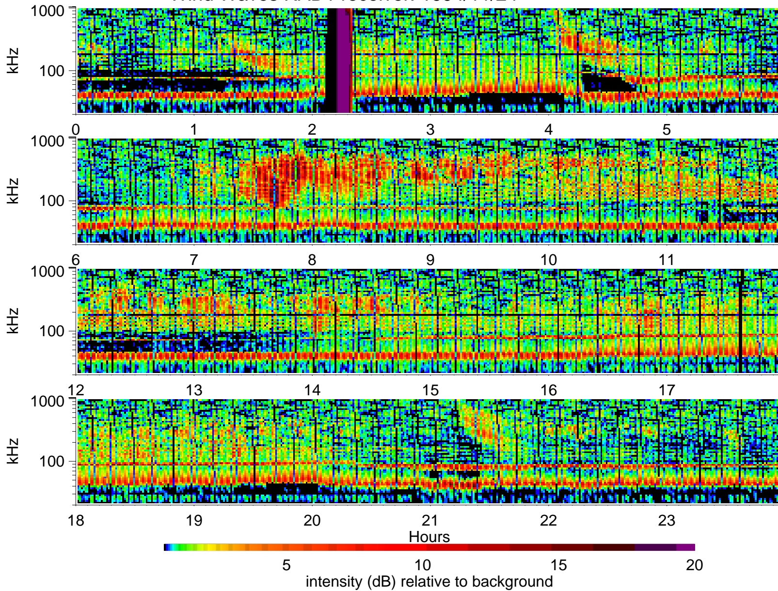
Wind Waves RAD1 receiver: 1994/11/24
