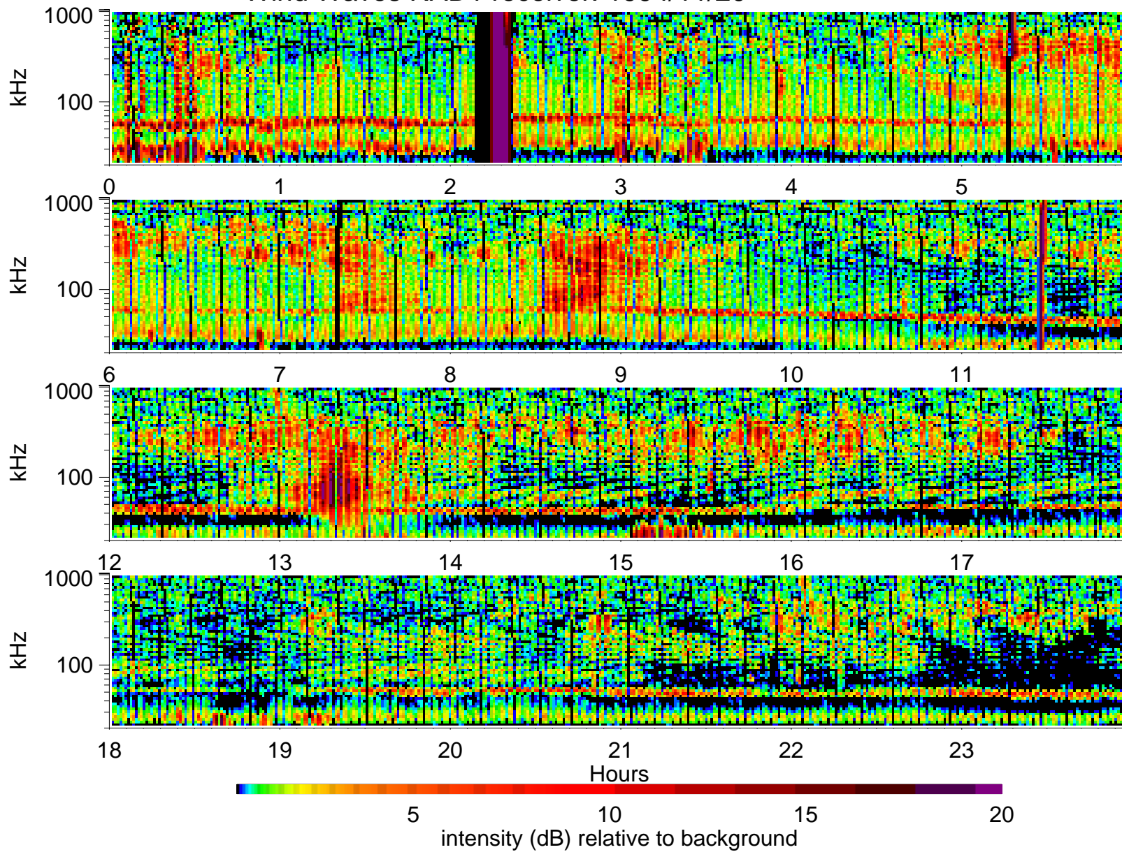
Wind Waves RAD1 receiver: 1994/11/20
