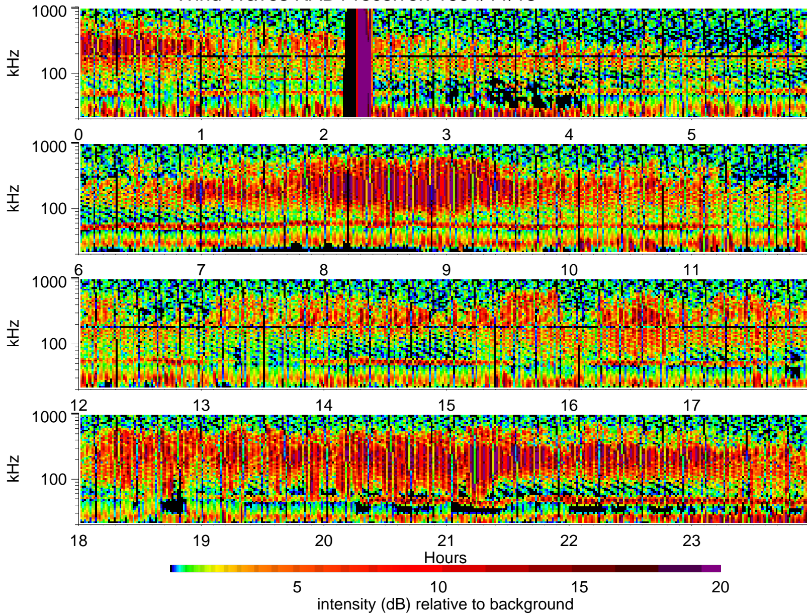
Wind Waves RAD1 receiver: 1994/11/15
