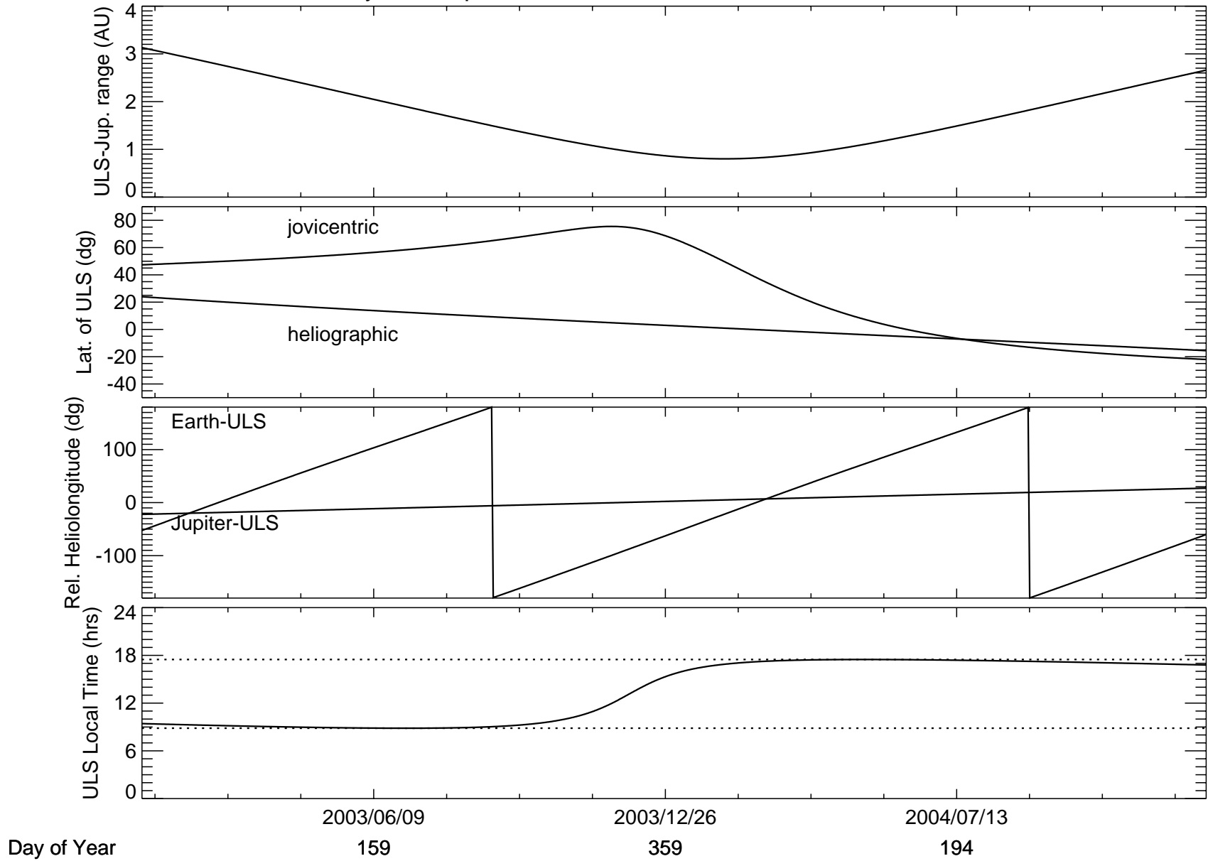
Ulysses/Jupiter/Earth coordinates: 2003/01/01-2004/12/31
