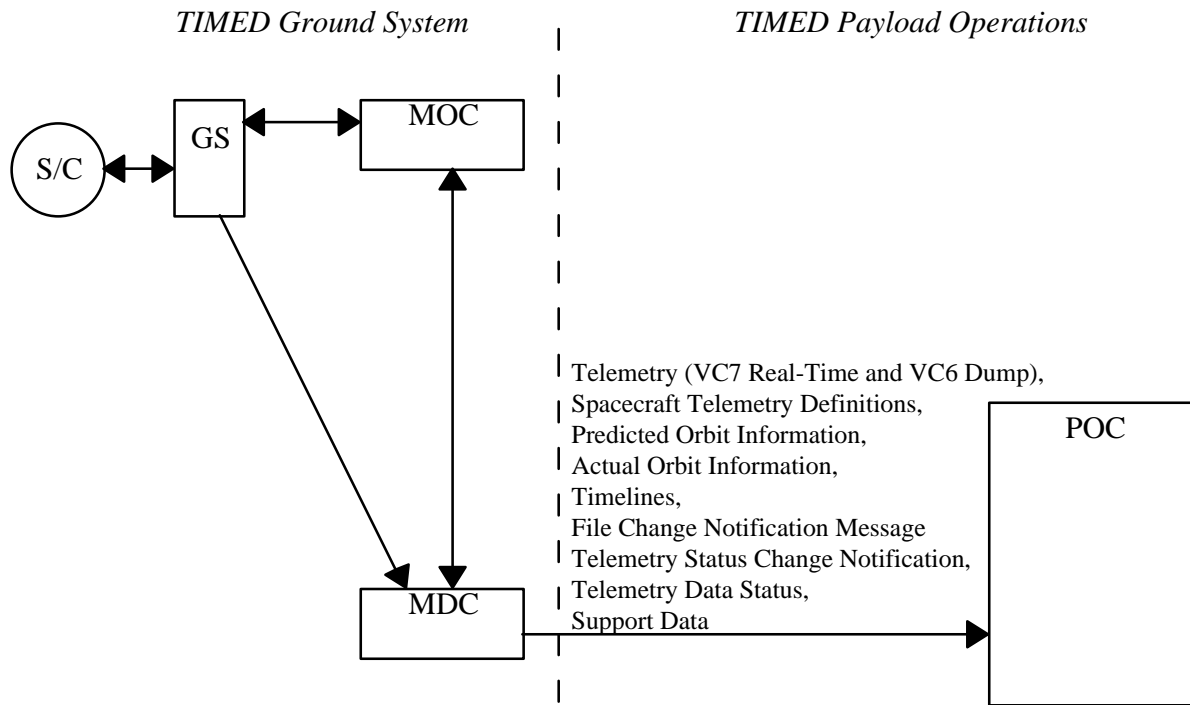
Figure 8.2.5-1. Mission Data Center to Payload Operations Center Interfaces
