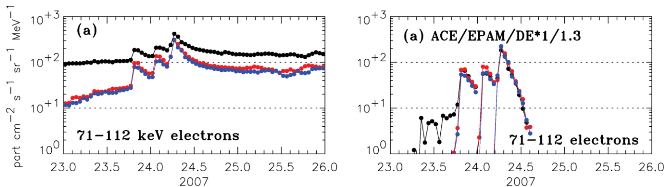
Fig. 1. Time profiles of three consecutive SEP electron events observed by STEREO-B, STEREO-A and ACE during 23-24 January 2007 when all three s/c were close to each other by s/c separation of less than 0.014 AU. Left panel: hourly averages of 71-112 keV electron intensity during 23-24 January 2007 events obtained by ACE(EPAM (black), STEREO-A (red) and STEREO-B (blue)). The right panel shows the same data as the left panel after pre-event intensity subtraction and application of the indicated multiplicative factor.
