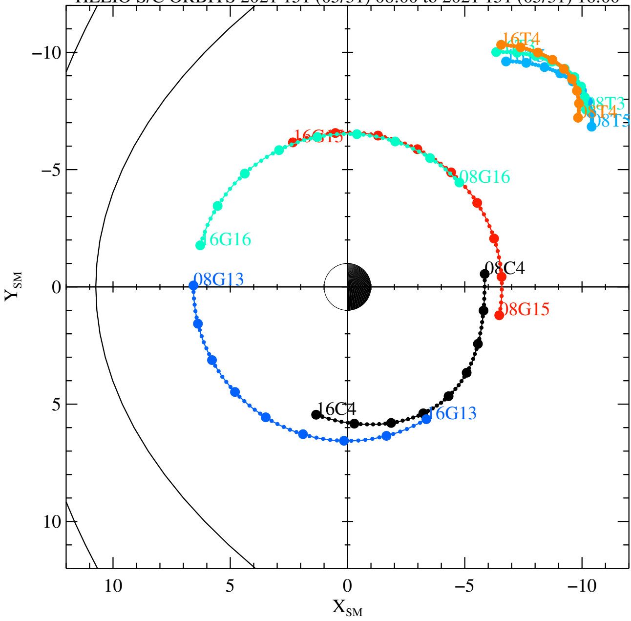
HELIO S/C ORBITS 2021 151 (05/31) 08:00 to 2021 151 (05/31) 16:00
