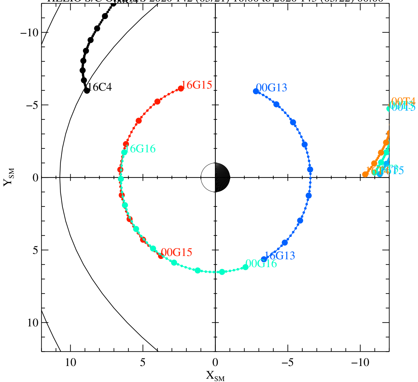
HELIO S/C ORBITS 2020 142 (05/21) 16:00 to 2020 143 (05/22) 00:00
