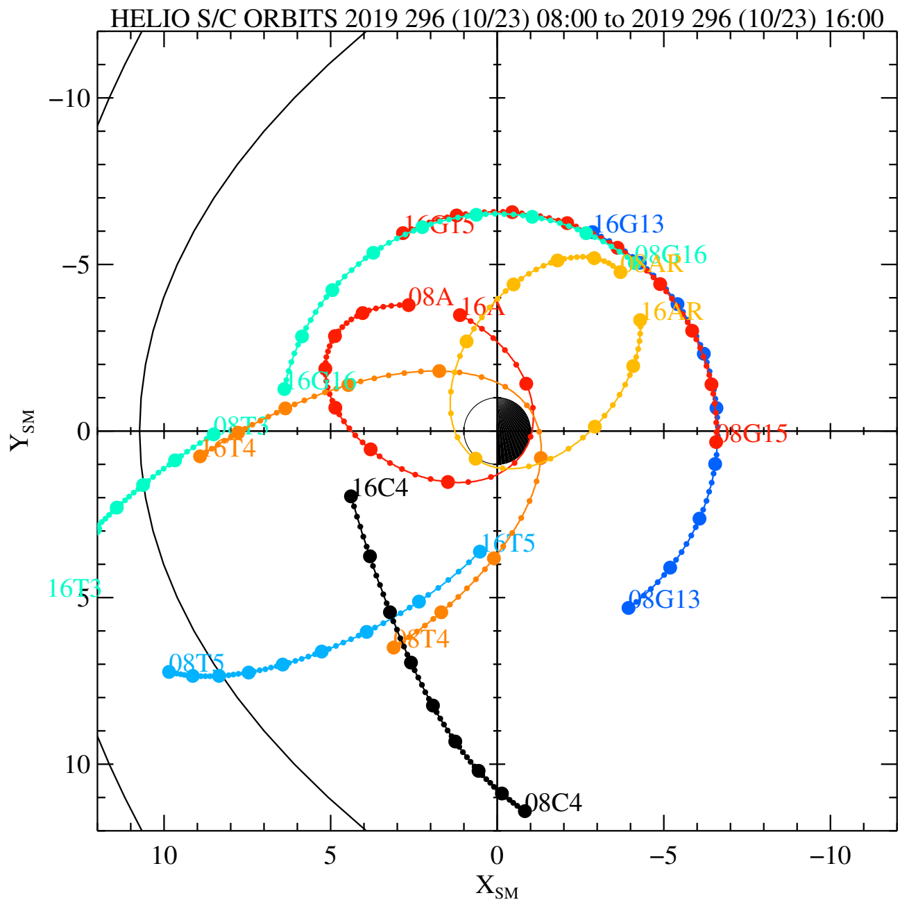
RBSPA-A, RBSPB-B, THEMISA-T5, THEMISD-T3, THEMISE-T4, CLUSTER4-C4, GOES13-G13, GOES15-G15, GOES16-G16, MMS1-MMS1, GEO
