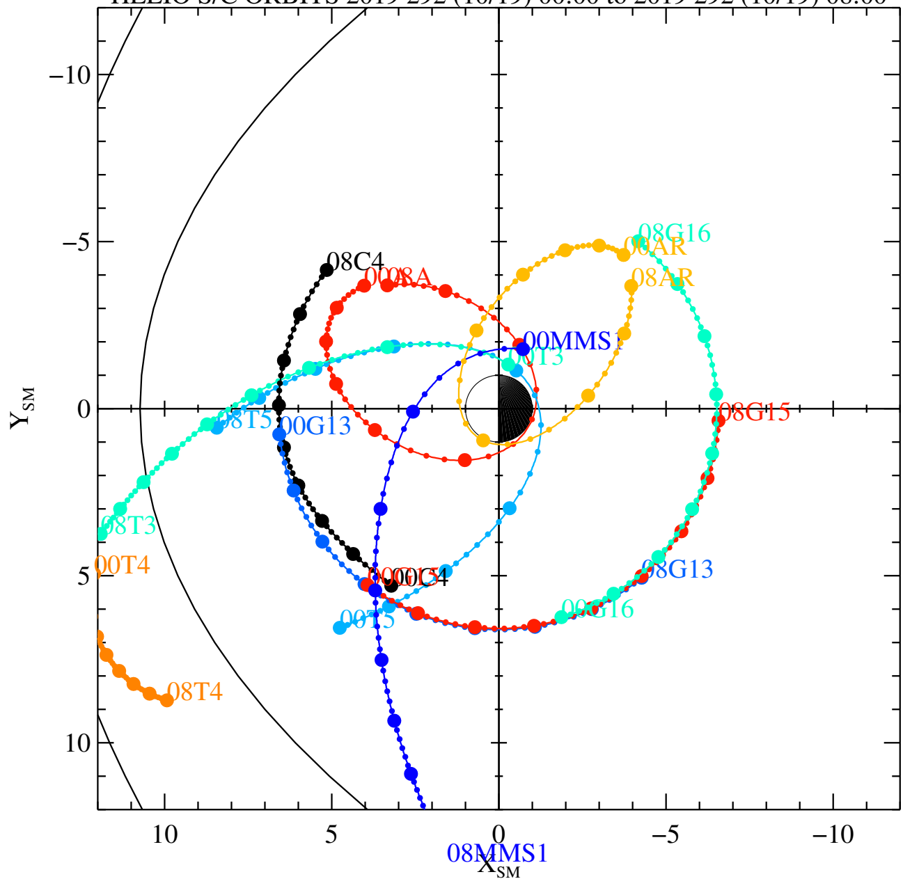
HELIO S/C ORBITS 2019 292 (10/19) 00:00 to 2019 292 (10/19) 08:00
