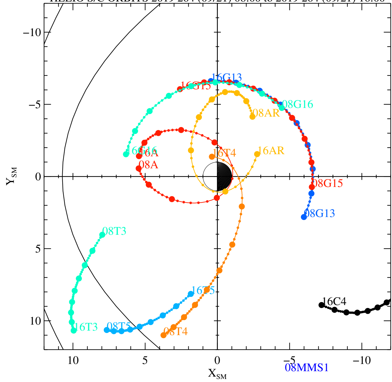
HELIO S/C ORBITS 2019 264 (09/21) 08:00 to 2019 264 (09/21) 16:00
