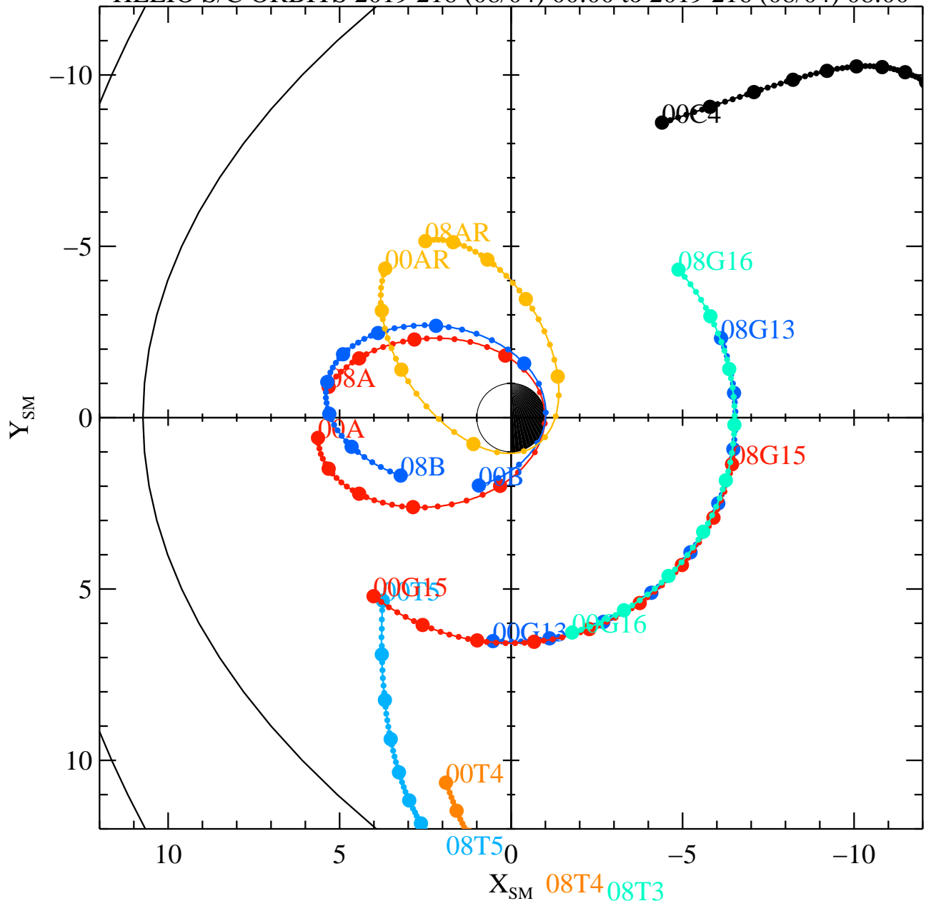
HELIO S/C ORBITS 2019 216 (08/04) 00:00 to 2019 216 (08/04) 08:00
