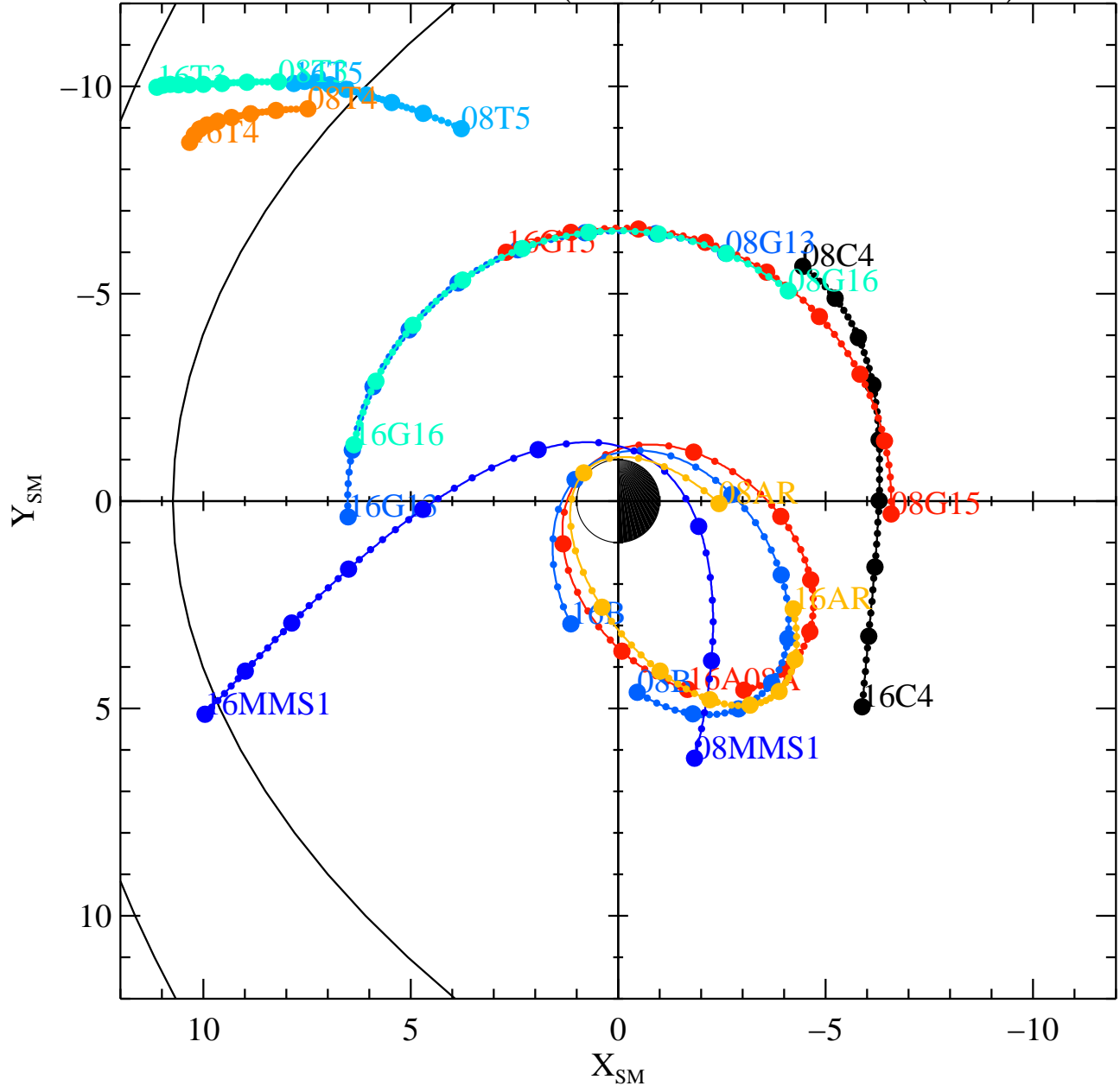
HELIO S/C ORBITS 2018 336 (12/02) 08:00 to 2018 336 (12/02) 16:00
