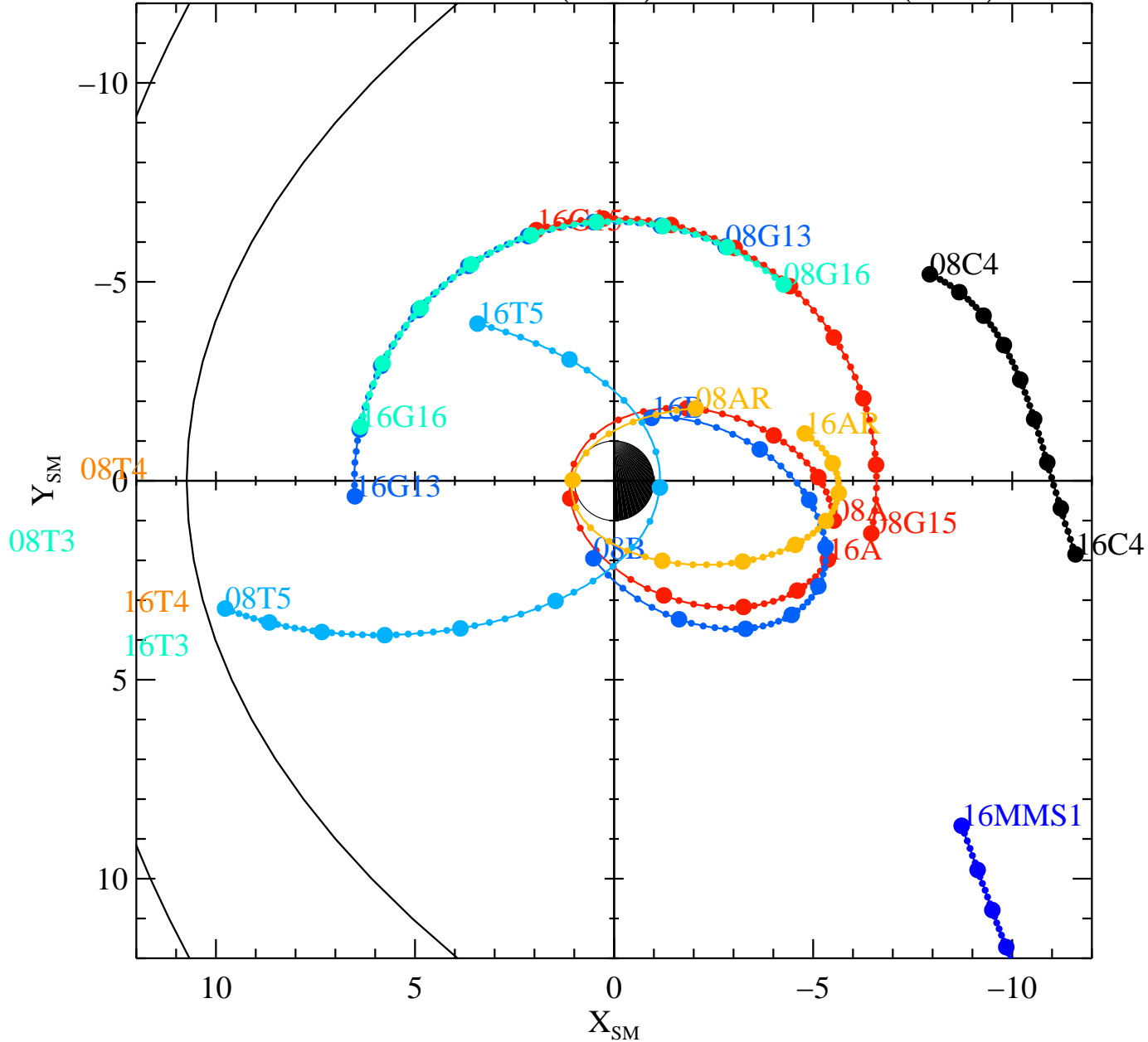
HELIO S/C ORBITS 2018 282 (10/09) 08:00 to 2018 282 (10/09) 16:00
