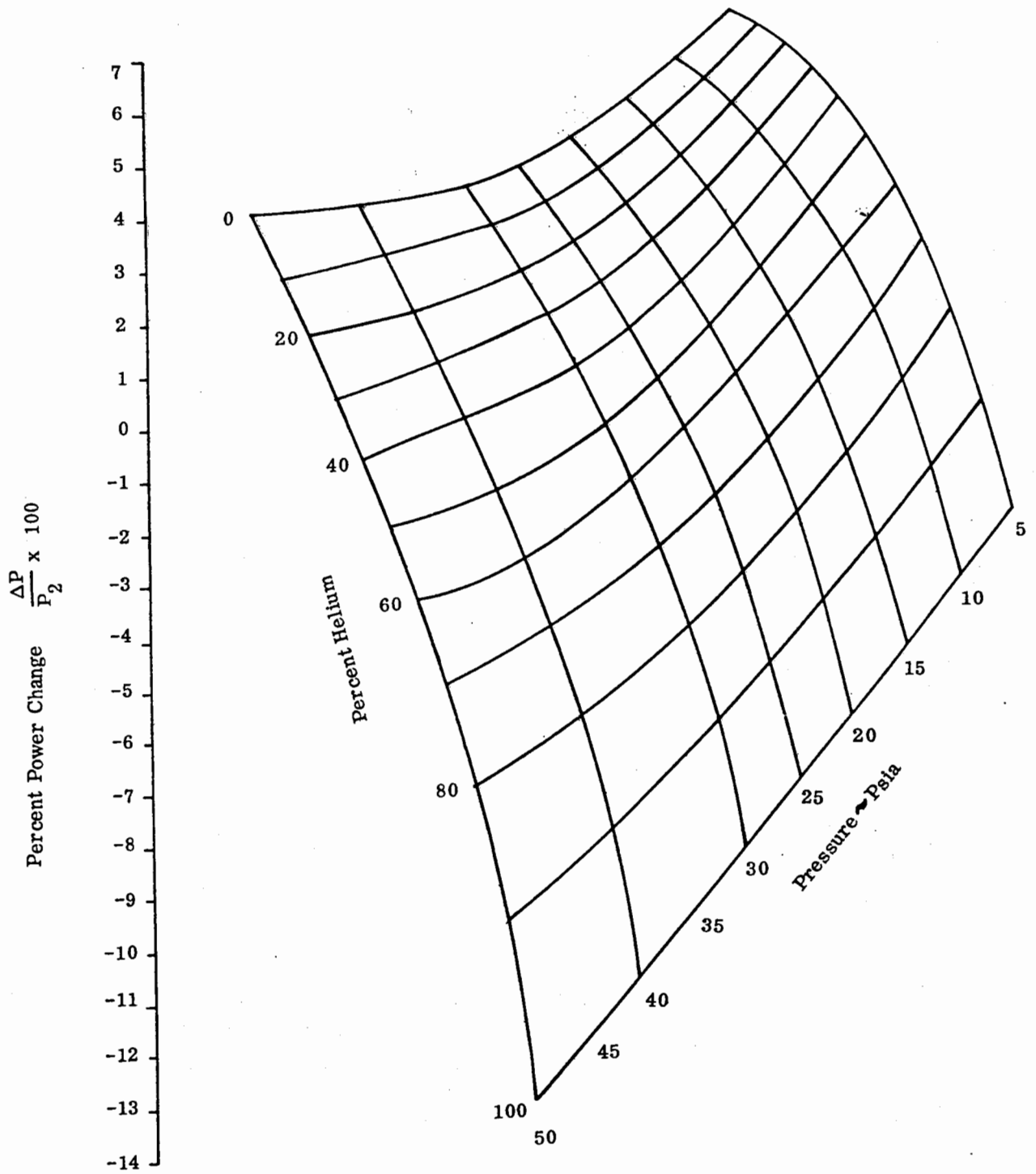
FIG. IV-6. S/N 41 POWER CHANGE WITH GAS COMPOSITION AND PRESSURE
