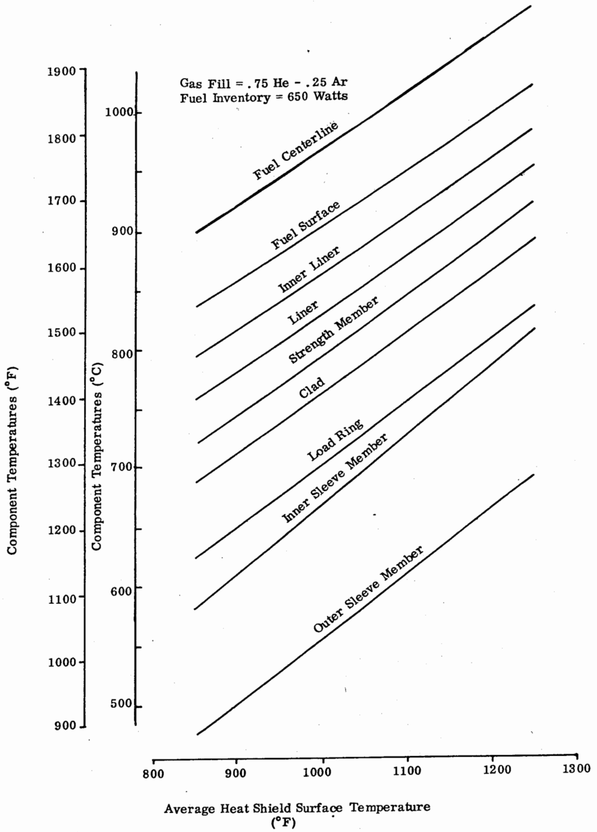
FIG. IV-24. MAXIMUM HEAT SOURCE TEMPERATURES
