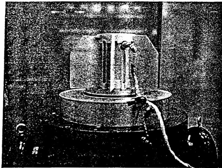
RTG S/N 52 WITH SHAKER VERTICAL (SPACECRAFT LATERAL 2 AXIS)
