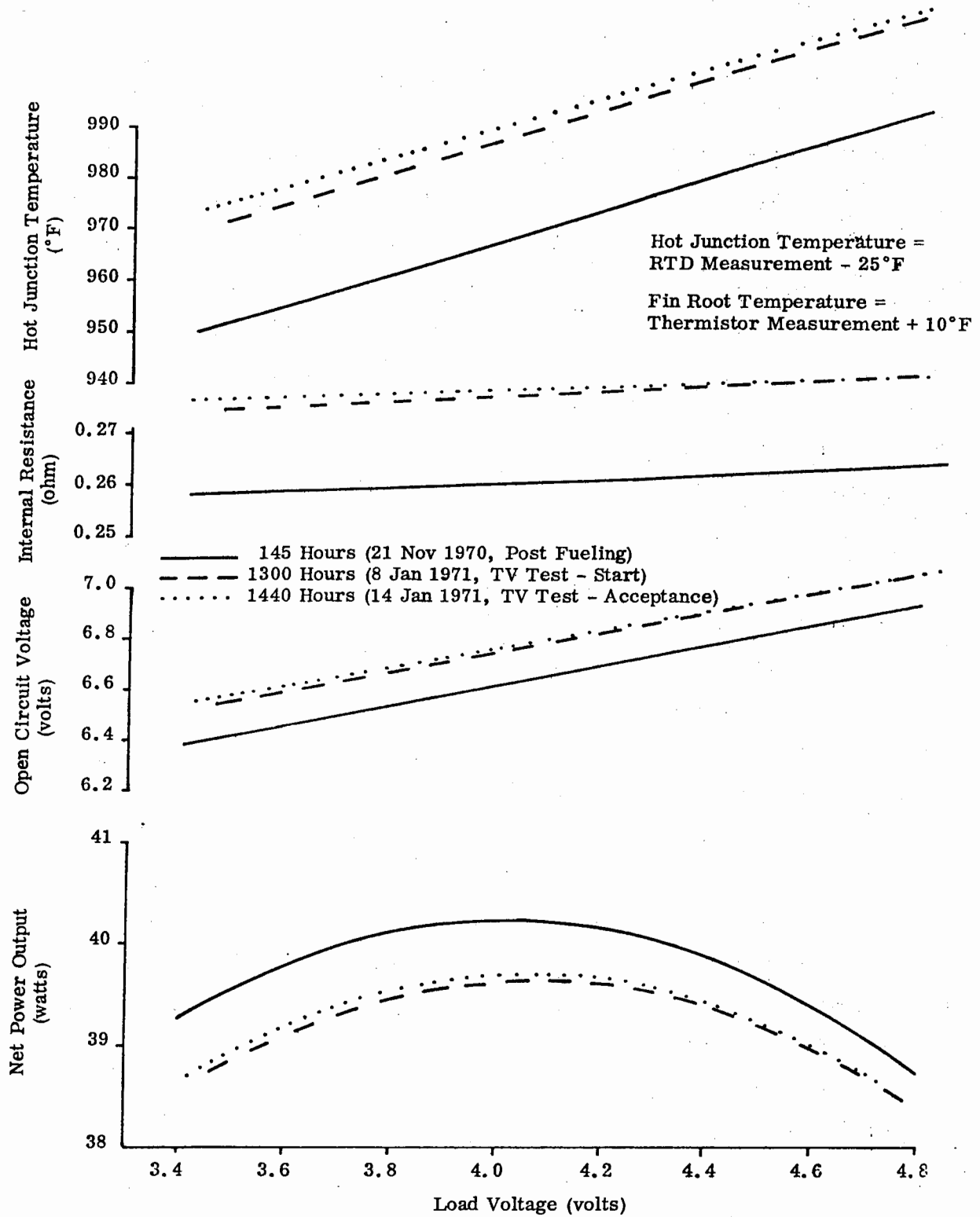
FIG. V-1. PARAMETRIC TEST RESULTS, SNAP 19 GENERATOR S/N 37 FIN ROOT TEMPERATURE: 330°F 644 WATTS (CAPSULE INVENTORY) FILL GAS: 75% HELIUM/25% ARGON
