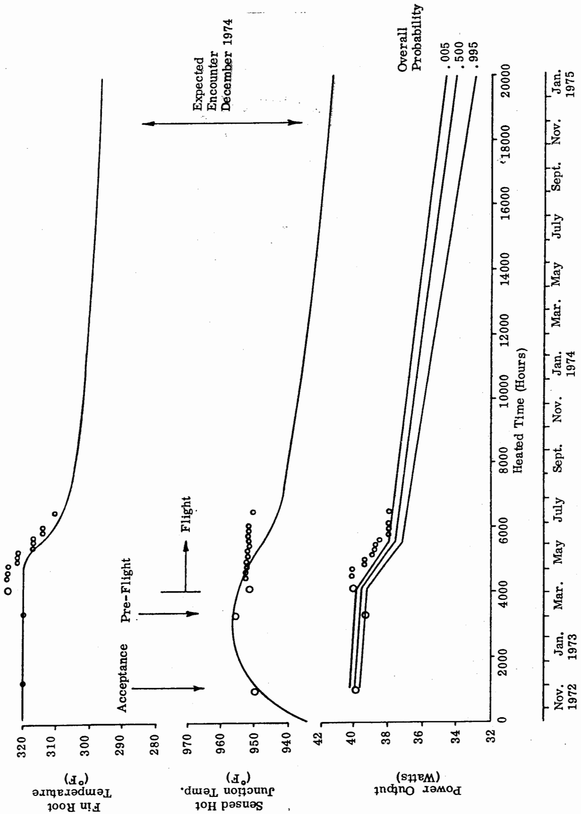
FIG. IV-16. PIONEER 11 RTG S/N 53 (INBOARD) PERFORMANCE
