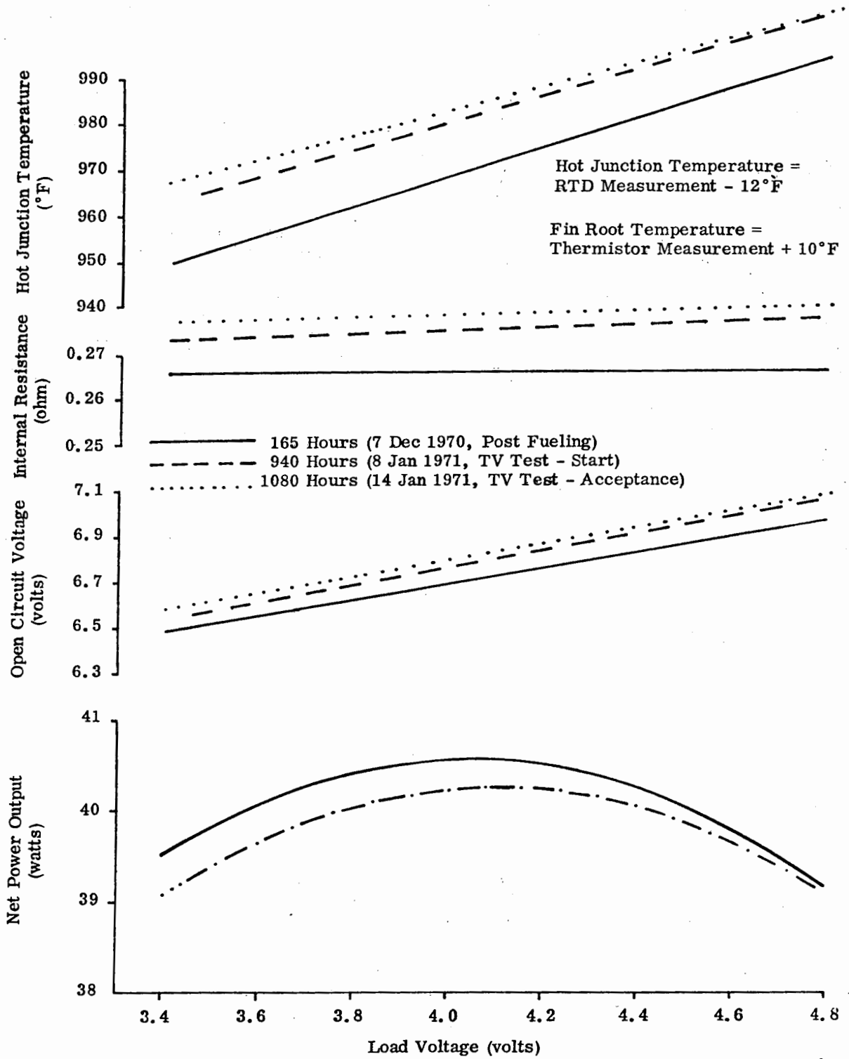
FIG. V-2. PARAMETRIC TEST RESULTS, SNAP 19 GENERATOR S/N 38 FIN ROOT TEMPERATURE: 330°F 647 WATTS (CAPSULE INVENTORY) FILL GAS: 75% HELIUM/25% ARGON
