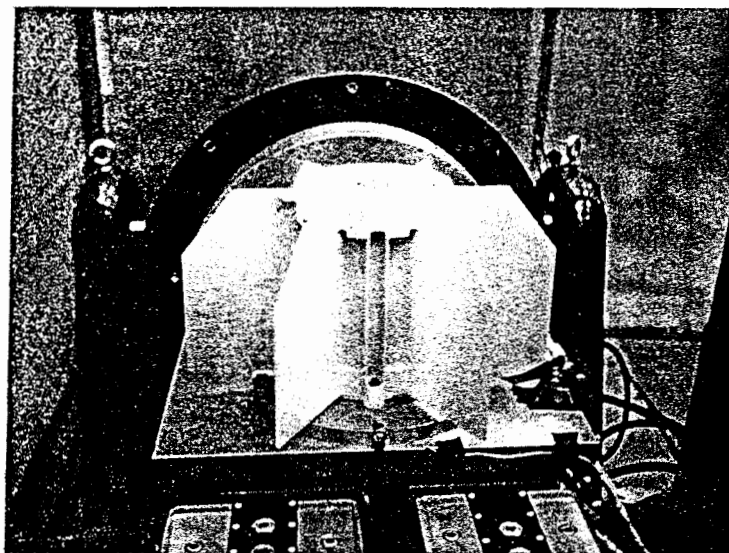
RTG S/N 53 WITH SHAKER HORIZONTAL (SPACECRAFT LATERAL 1 AXIS)
