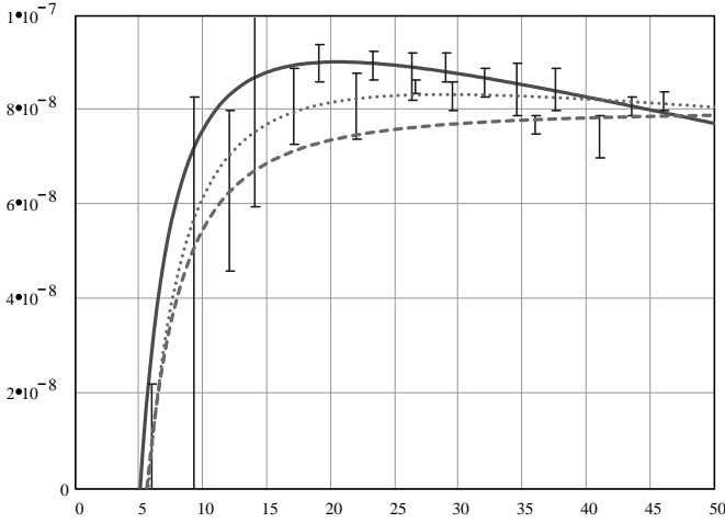
FIG. 8: Data from Figure 1 (error bars), model prediction from this paper (solid line), pure 88 year half life plus solar constant error (middle line), and constant acceleration plus solar constant error (lowest line)
