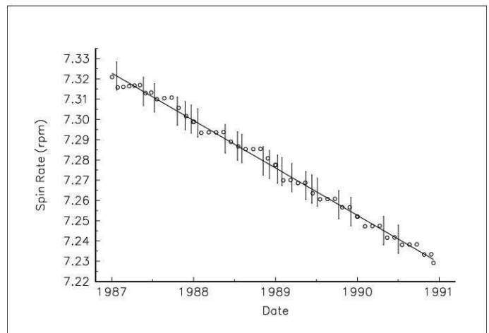
FIG. 4: Spin changes in Pioneer 11 [1]. The vertical lines indicate the times of maneuvers.
