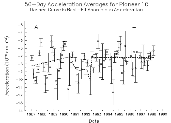
FIG. 2: Unmodelled acceleration and an empirical fit from Turyshev[4].
