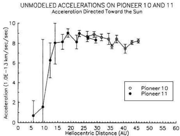
FIG. 2: Unmodelled acceleration and an empirical fit from Turyshev[4].
