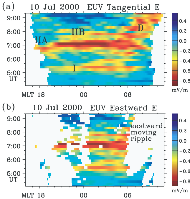
Figure 3. Electric field inferred from IMAGE EUV, 10 July 2000. (a) E_{\pi} (E-field tangent to the moving plasmopause boundary) versus UT and MLT. Colorbar gives strength in mV/m, saturated at -0.9 mV/m. (White = no data.) (b) E_{\varphi} (azimuthal E-field) estimated from E_{\pi} for cases in which \alpha \leq 8^{\circ} , where \cos \alpha \equiv (\hat{\pi} \cdot \hat{\varphi}) .
