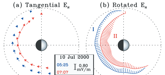
Figure 2. Equatorial plots showing EUV electric field tangential to the plasmopause at 5:25 UT (blue) and 7:07 UT (red) on 10 July 2000. (a) Tangential electric field vectors, scaled as 1 R_E = 0.8 \text{ mV/m} . (b) Scaled flow-directions at plasmopause ( E_\pi vectors rotated 90^\circ ).
