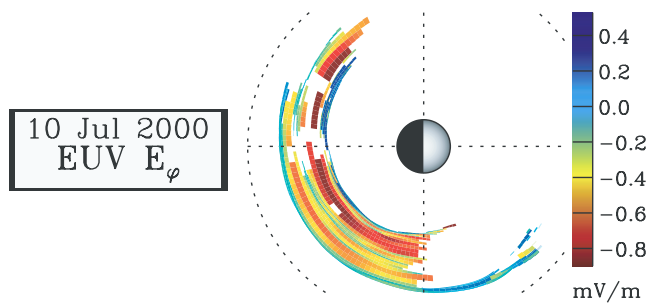
Figure 4. Azimuthal electric field component E_\phi inferred from IMAGE EUV observations, 10 July 2000, plotted in the equatorial plane (Earth at center; Sun to right). The dotted circle is at geosynchronous orbit. Colorbar gives E_\phi strength in mV/m.
