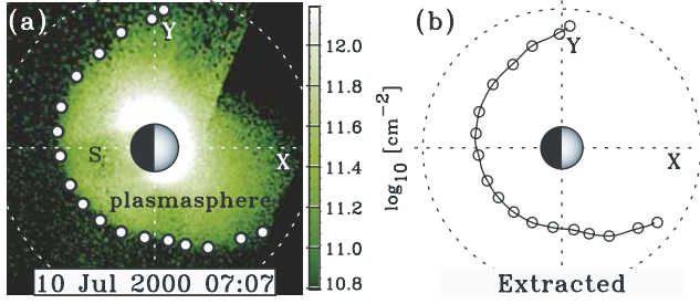
Figure 1. Example of extraction of plasmopause curve from IMAGE EUV, 10 July 2000, 7:07 UT. (a) EUV image, mapped to the magnetic equator (Earth at center; Sun to the right). Dotted lines are X - and Y -axes; dotted circle is geosynchronous orbit. The colorbar gives line-of-sight integrated \text{He}^+ column abundance. Black region in upper right is sunlight contamination. Filled white circles are manually-extracted ('click') points along the plasmopause. (b) Fourier expansion of the click points (circles) is plotted as the solid curve.
