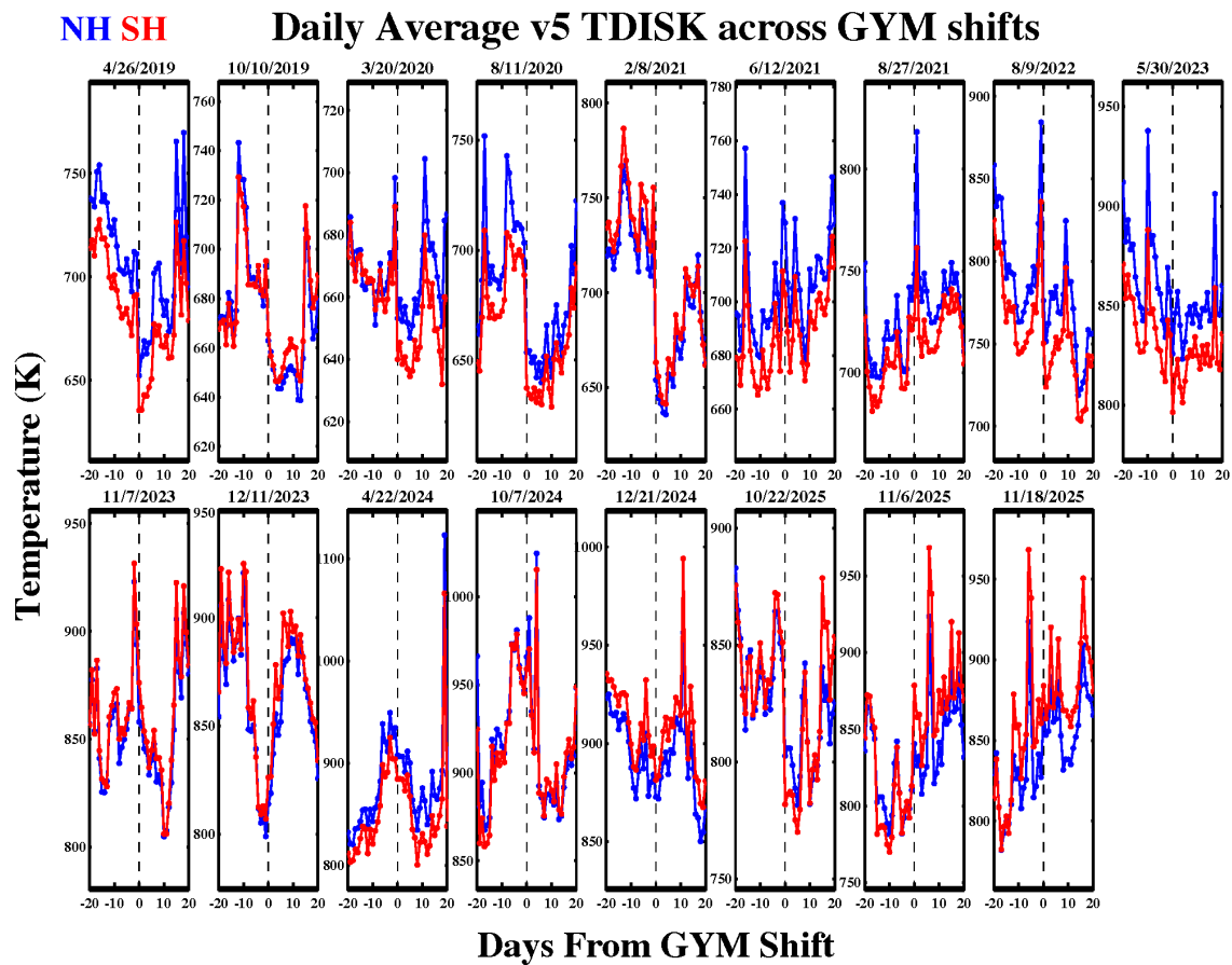
Figure 3-20 Daily average TDISK v05 data before and after the Channel A GYM shift operations to date. Northern/Southern hemisphere (NH/SH) are plotted in blue and red, respectively. In each panel the vertical line is the date of the GYM operation.
