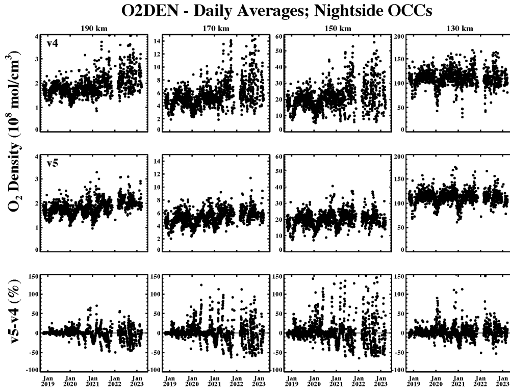
Figure 2-12 Daily average O2DEN data from nightside occultations at 4 altitudes (columns)
