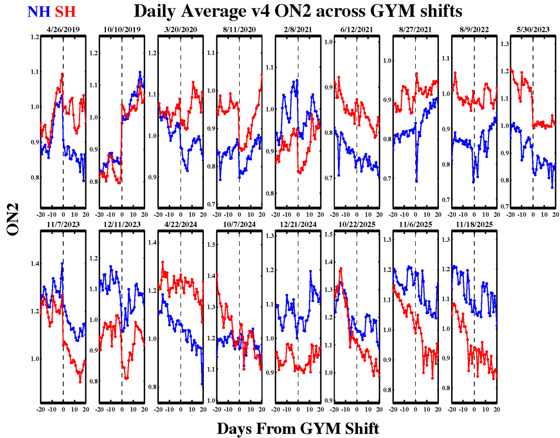
Figure 3-21 Daily average v04 ON2 data before and after the Channel A GYM shift operations to date. Northern/Southern hemisphere (NH/SH) are plotted in blue and red, respectively. In each panel the vertical line is the date of the GYM operation.
