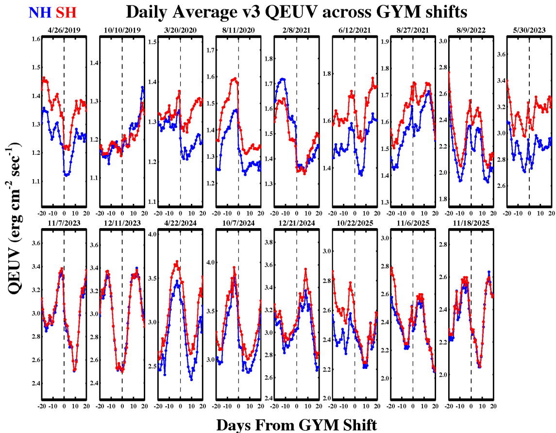
Figure 3-23 Daily average v03 QEUV data before and after the Channel A GYM shift operations to date. Northern/Southern hemisphere (NH/SH) are plotted in blue and red, respectively. In each panel the vertical line is the date of the GYM operation.
