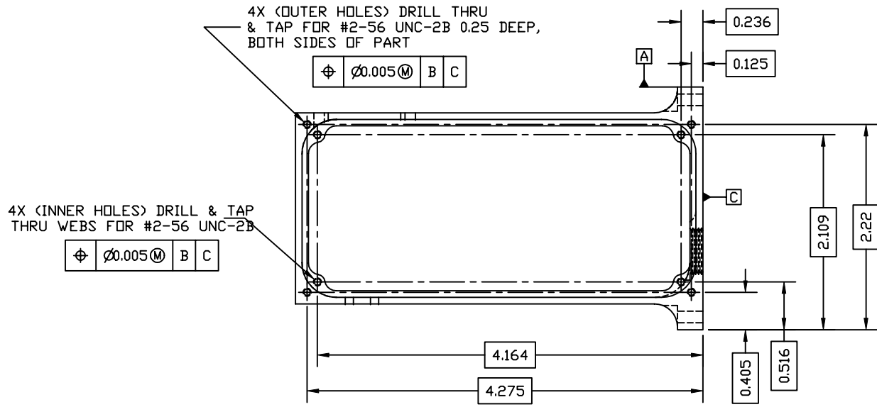
VIEW B-B
