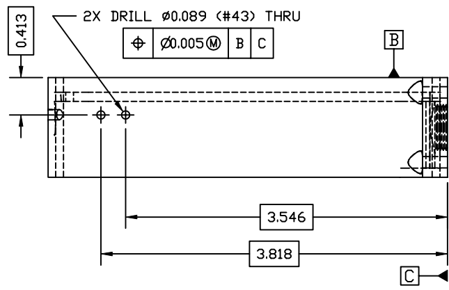
VIEW B-B
