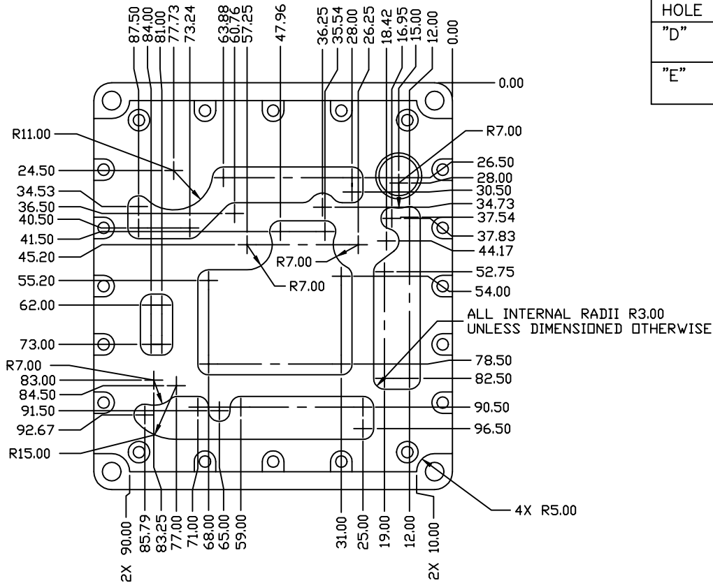
VIEW K-K (HIDDEN LINES, FEATURES IN DETAILS "H" AND "J", AND TAPPED HOLES REMOVED FOR CLARITY)
