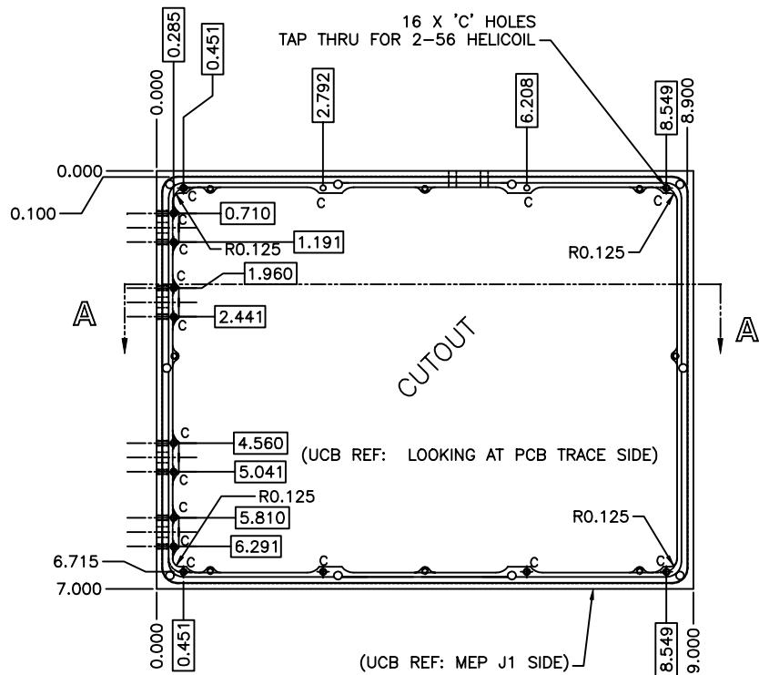
VIEW C-C
