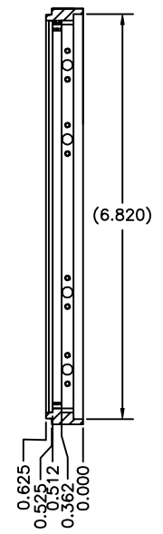
SECTION B-B
