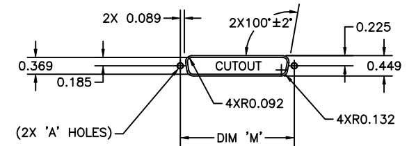
CONNECTOR CUTOUTS DETAIL
