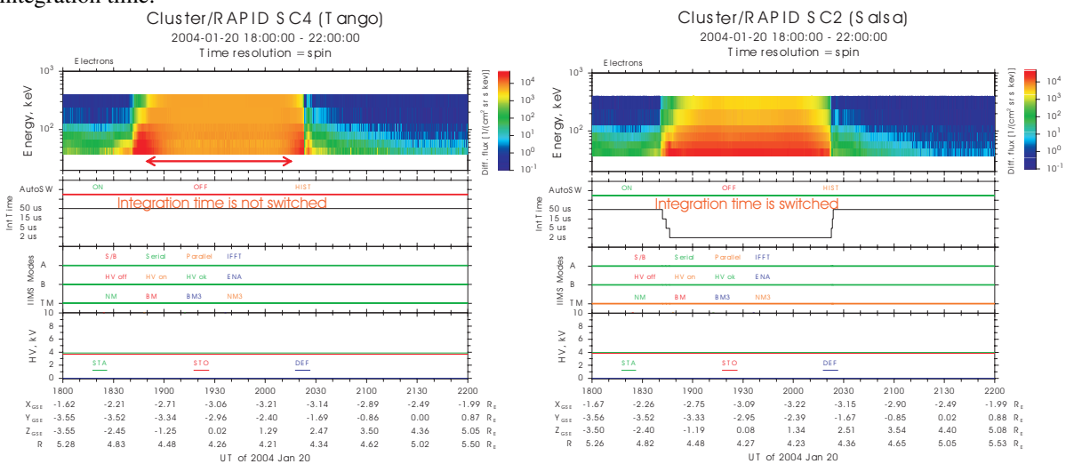
Figure 6: Left: An illustration of what can happen when the integration time fails to switch. As the intensities increase, the count rates in the lowest channels are too low, since multiple low-energy events count as a single high-energy one. Right: For a comparison the same time period and the same region measured by another Cluster spacecraft where the auto-switching was working properly.
