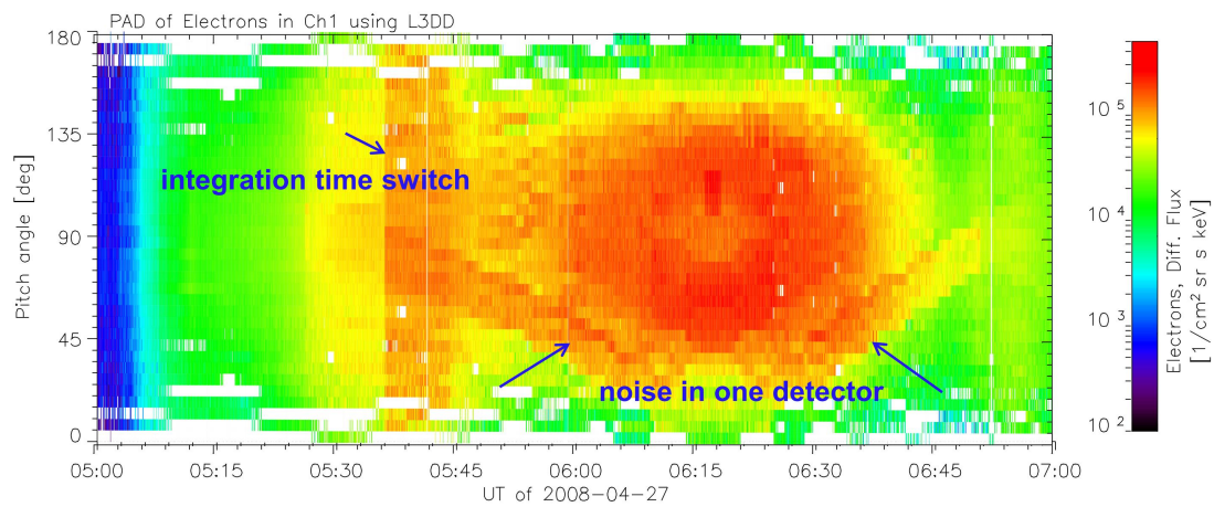
Figure 12: An example of the electron data contamination in the radiation belts. In the pitch-angle distribution of the electrons one could see stripes denoted as the noise in one detector. The fact that this noise appears only in the radiation belts implies that the contamination is from penetrating particles. The sharp enhancement of the electron flux at the integration time switch is not related to the contamination problem.
