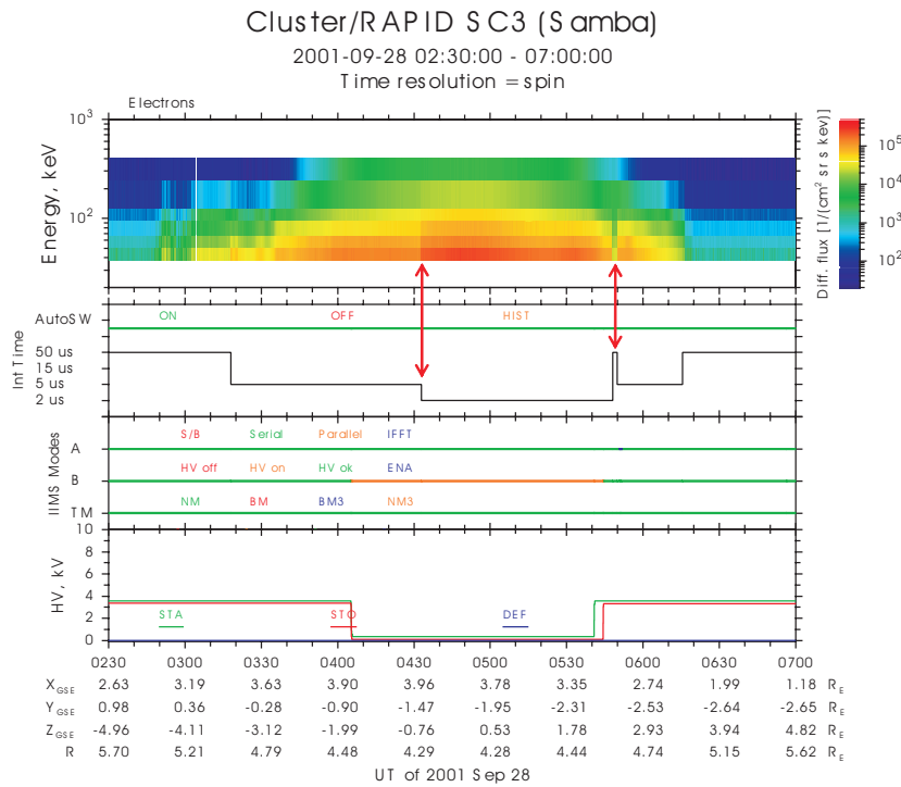
Figure 5: Demonstration of how changes in the IES integration times can produce erroneous changes in the electron fluxes if the automatic switching occurs too late (times are denoted by red arrows). For example at ~04:32 integration time (second from the top panel) switches from 5 \mu s to 2 \mu s and produces the sudden sharp change in the electron intensity. Another example one can see at ~05:49, when integration time was erroneously switched from 2 \mu s to 50 \mu s and than back to 5 \mu s producing a sharp intensity drop for the time of the too-long integration time.
