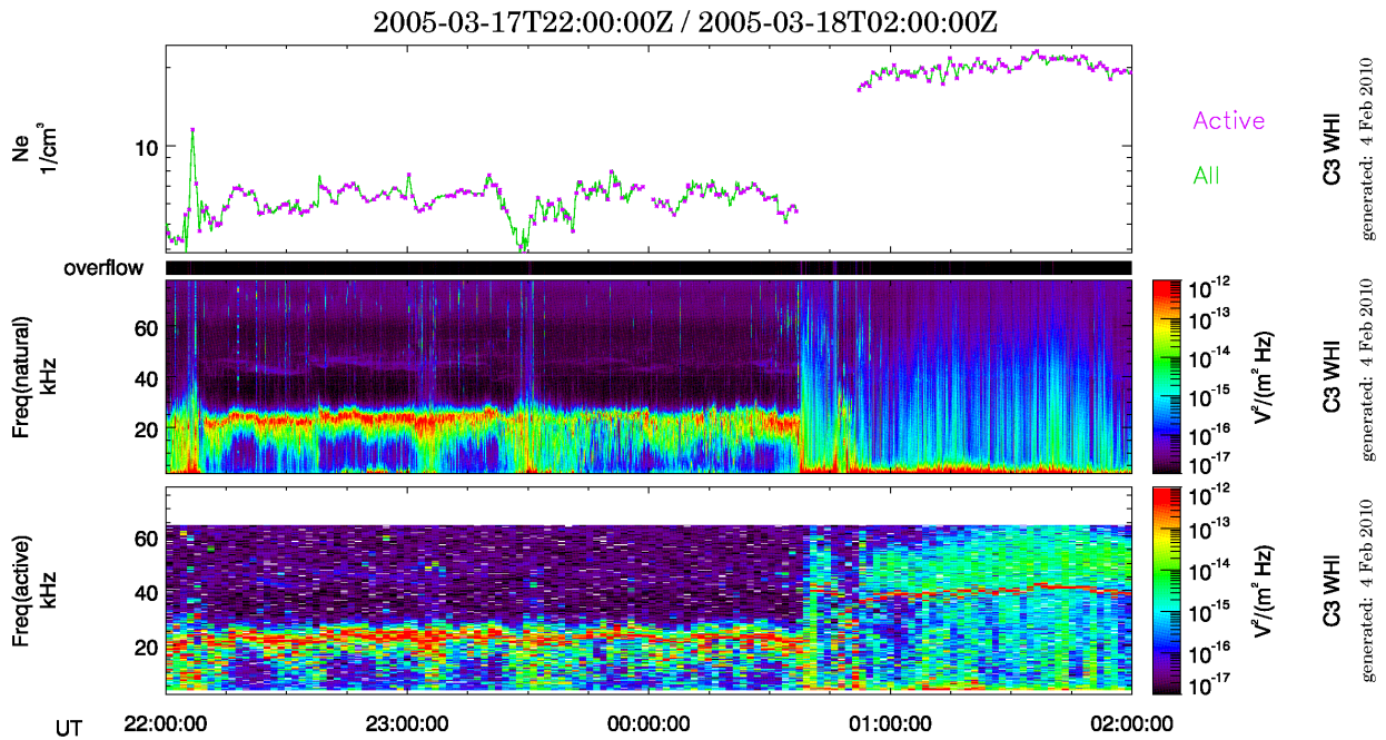
Figure 5: Example of density values and NATURAL and ACTIVE spectrograms (from top to bottom) for C3 on March 17, 2005, corresponding to solar wind/magnetosheath transition. Density values extracted from the ACTIVE WHISPER spectra are plotted as purple points whereas green line represents the density extracted from both ACTIVE and NATURAL measurements. In this interval two methods were used: Max2_EFW for ACTIVE and Proxy_EFW for NATURAL.
