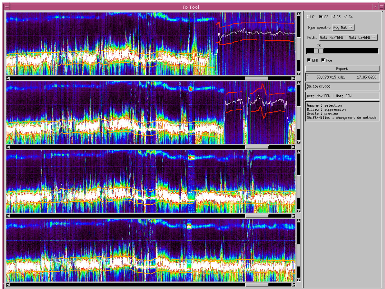
Figure A.1: Typical density processing session. On the left: WHISPER electric field spectrograms for the 4 spacecraft (the sliders allow scrolling through the whole spectrograms for 1 day). The orange and red bands are the search bands determined by the operator (the color indicates the algorithms that will be applied). The white line is the recalibrated EFW potential (the gyrofrequency can also be plotted). On the right: controls that allow to choose the spectrograms to handle, the current views (active, natural or average), the list of methods, and the search band width.
