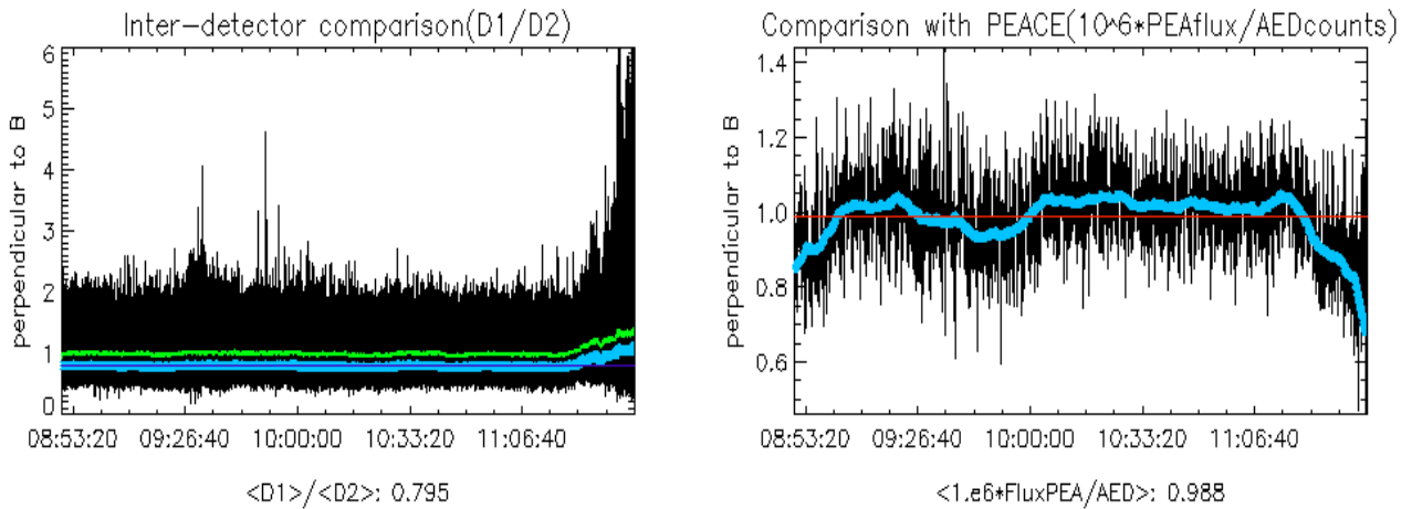
Figure 6.7. Inter-detector ( f_{id} – left panel) and calibration ( f_{cal} * 10^6 – right panel) factors for 22 October 2005, 08:50-11:40 UT. High resolution factors (thin black), averages over the PEACE acquisition time intervals ~4s (thick light blue) and medians of the factors for the same intervals (green line). The thin blue line in the left panel and the red line on the right are the mean values for the whole time interval.
