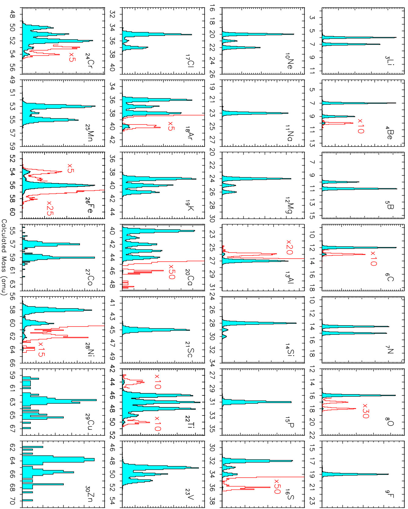
Cosmic Ray Mass Distributions Measured with ACE/CRIS at Solar Minimum (Dec 1997 through Sept 1999)
